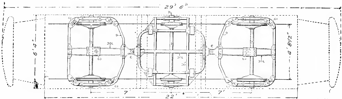
Fig. 5672. Plan of Truck on a Tangent.
